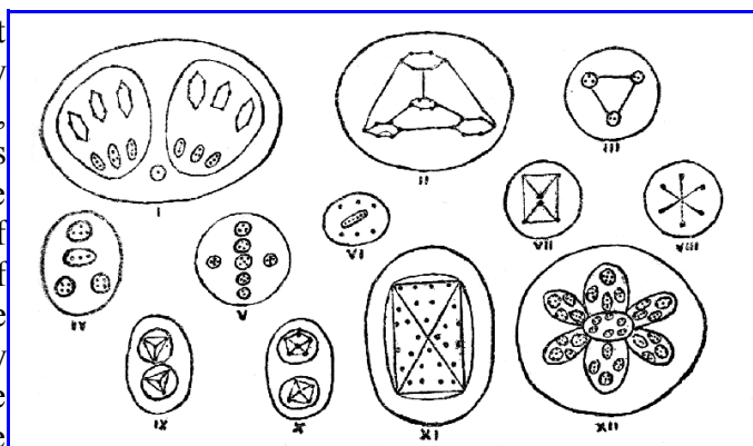
TYPES OF PROTO-ELEMENTAL MATTER.
