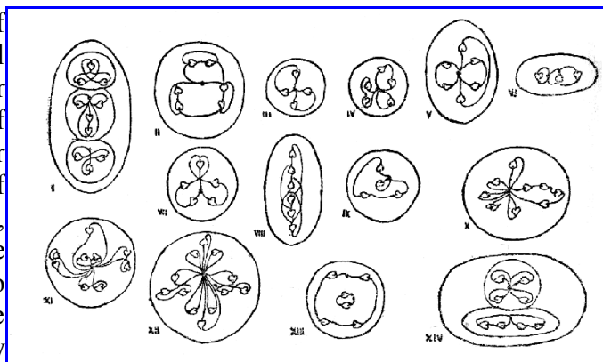
TYPES OF META-PROTO-ELEMENTAL MATTER.
