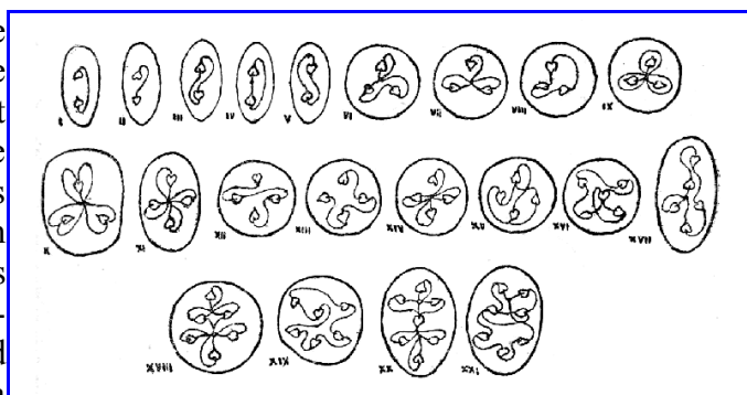
TYPES OF HYPER-META-PROTO-ELEMENTAL MATTER.
